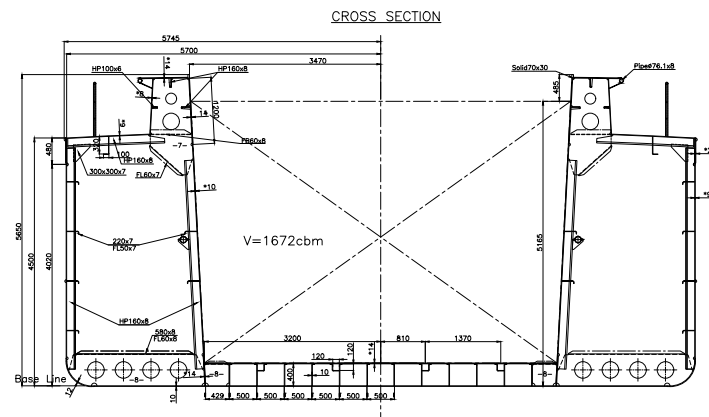
CROSS SECTION
